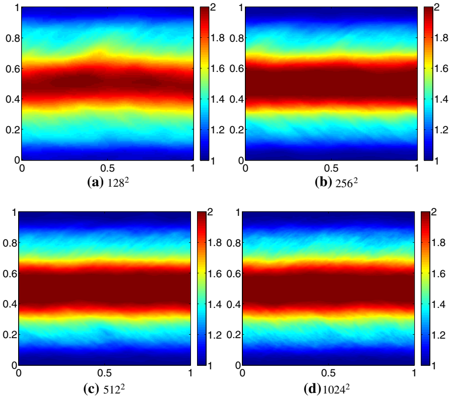
Fig. 8 Approximate sample means of the density for the Kelvin–Helmholtz problem (32) at time t = 2 and different mesh resolutions. All results are with 400 Monte Carlo samples
